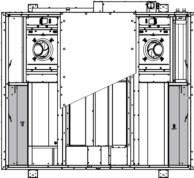
Abb. 14-2 Position Luftfilter
