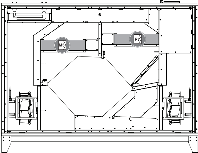
Abb. 14-2 Position Luftfilter
