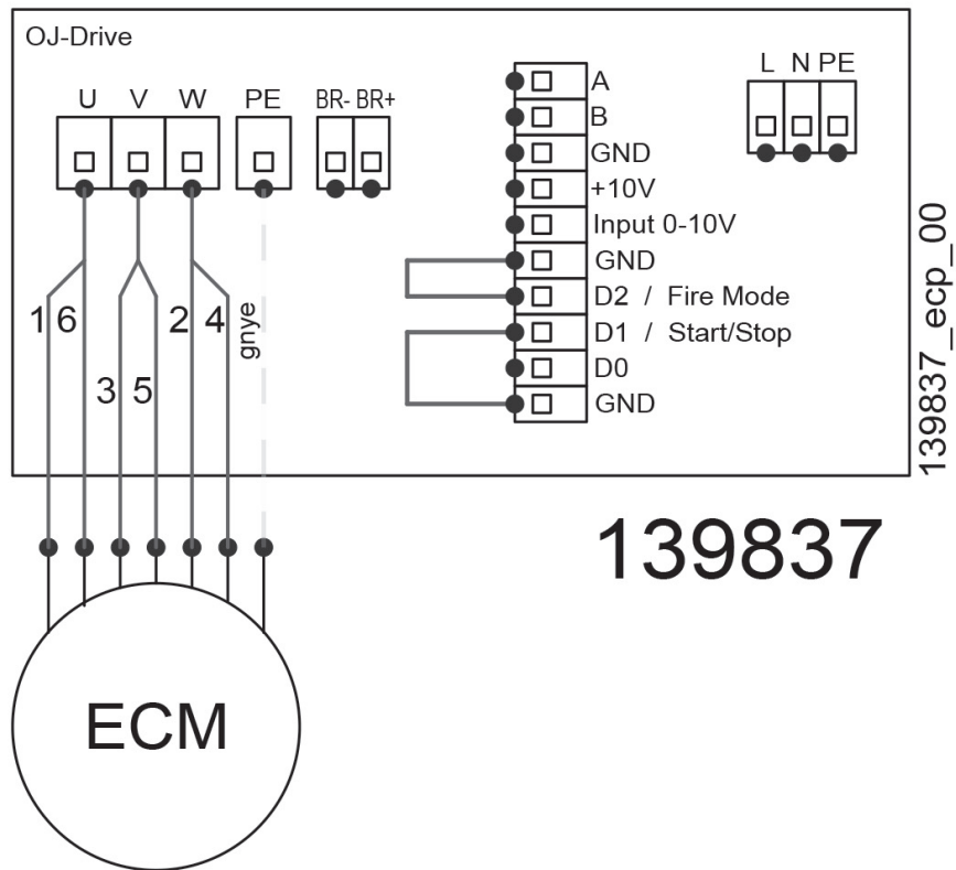
0-10V Signal
