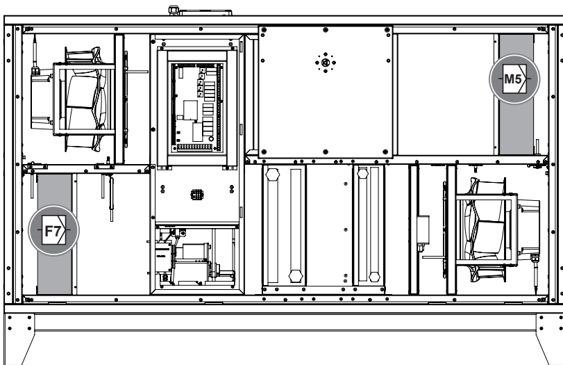
Abb. 14-7 Position Luftfilter
