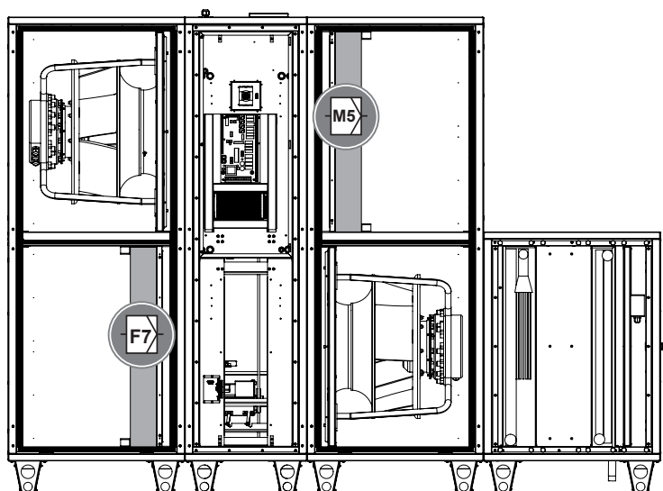
Abb. 14-7 Position Luftfilter
